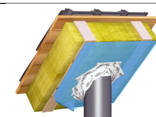
Abb. 5: Dunstrohr innen
