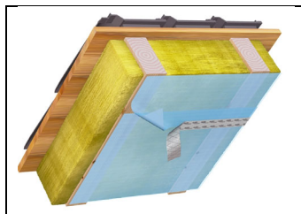
Abb. 4: Überlappung innen
